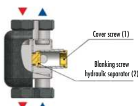
The MINI hydraulic separator The flow diagram between supply and return.
